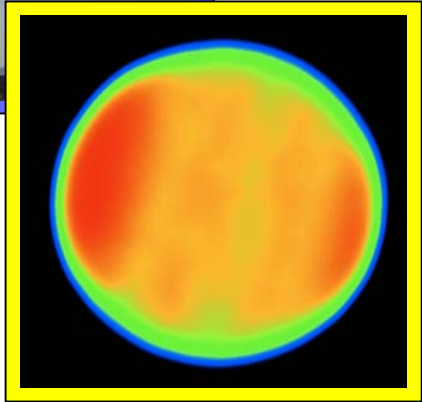
Uranus image taken by the VLA at K-band (1.3 cm). Notice the two hemispheres look symmetric
